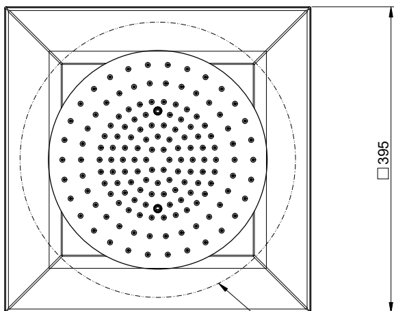
INSTALLATION MODE 1
