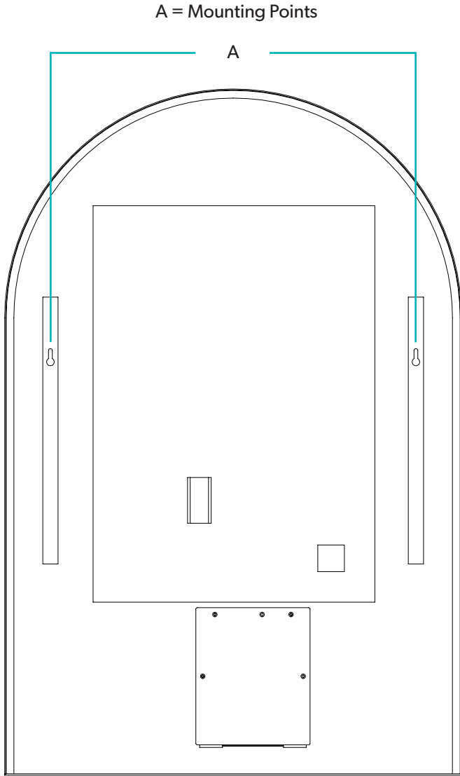
Fig 2. - Mounting points
